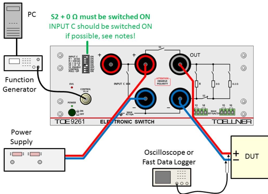
Fig. 9: Test assembly for VDA 320, E48-09
