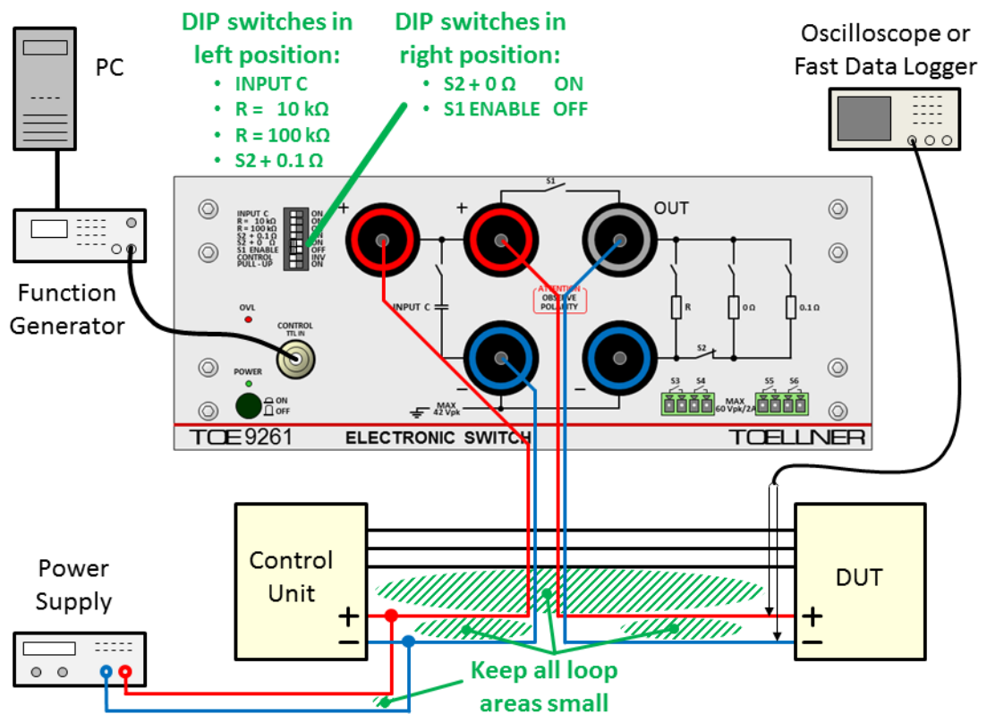
Fig. 7: Test assembly for LV 124, E-13; interruption of a ground pin > 4 A
