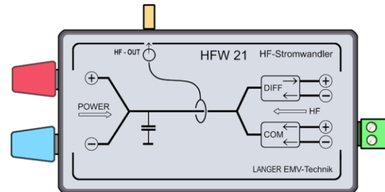
Figure 10 HFW 21 RF Current Transformer (schematic)
