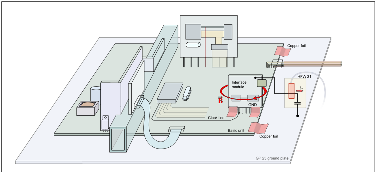
Figure 29 Evaluation of the modifications with the HFW 21
