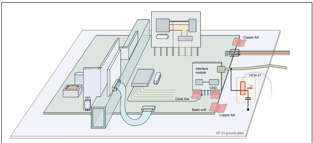
Figure 30 HFV 21 detects the voltage drop on the shield of the connected data cable
