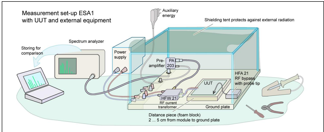
Figure 15 Measurement set-up ESA1 (schematic)
