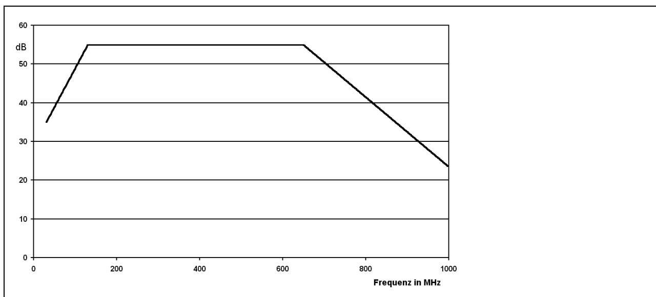
Figure 36 Approximate shield damping with the shielding tent closed
