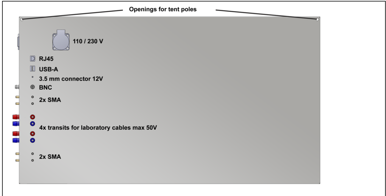
Figure 2 GP 23 Ground Plate
