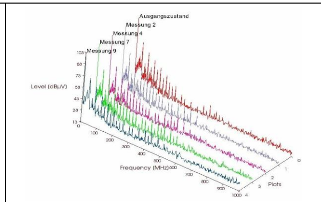
Figure 17 3D diagram
