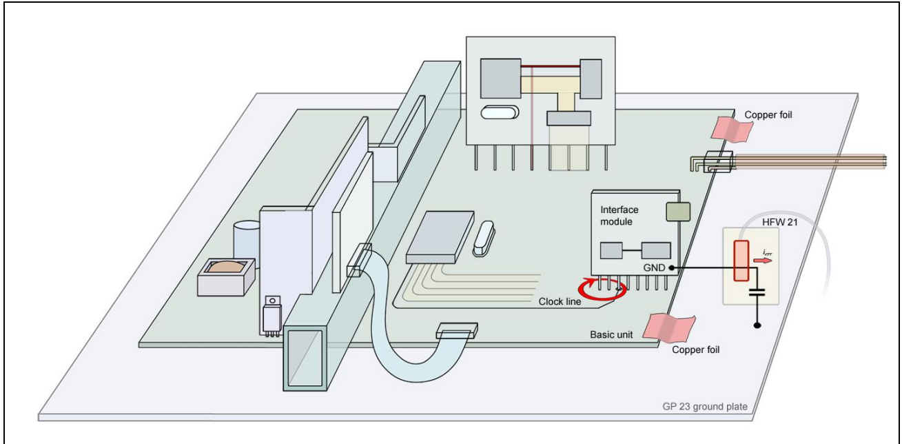
Figure 28 GND of the interface module connected to the COM output of the HFW 21
