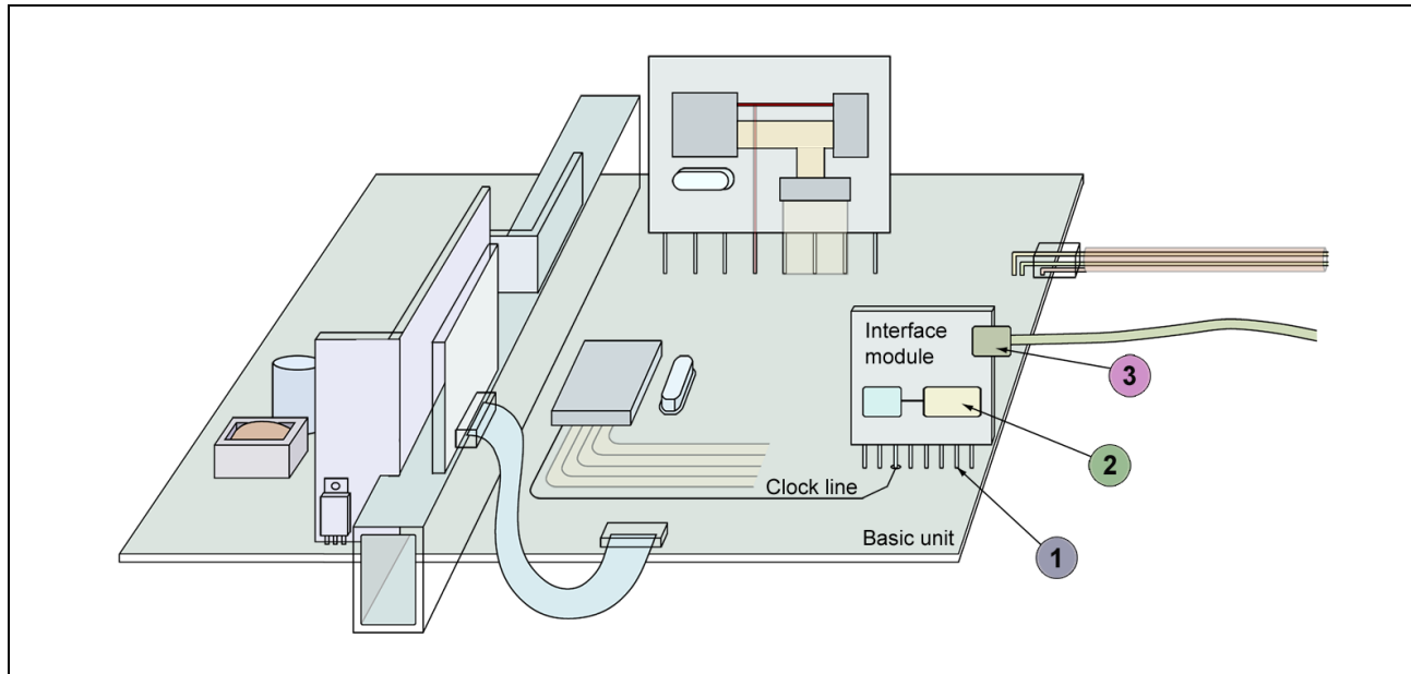
Figure 27 RF sources on the interface module
