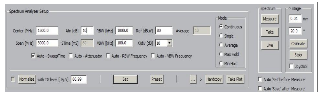
Figure 19 Spectrum Analyzer Setup
