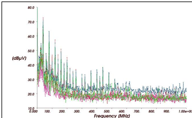
Figure 16 2D diagram
