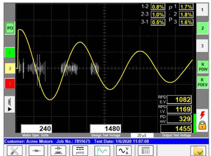
Partial Discharge Test
