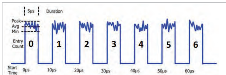
Example seven pulse waveform.
