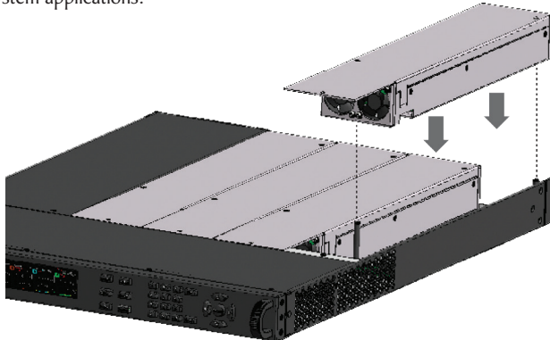
Module installation
